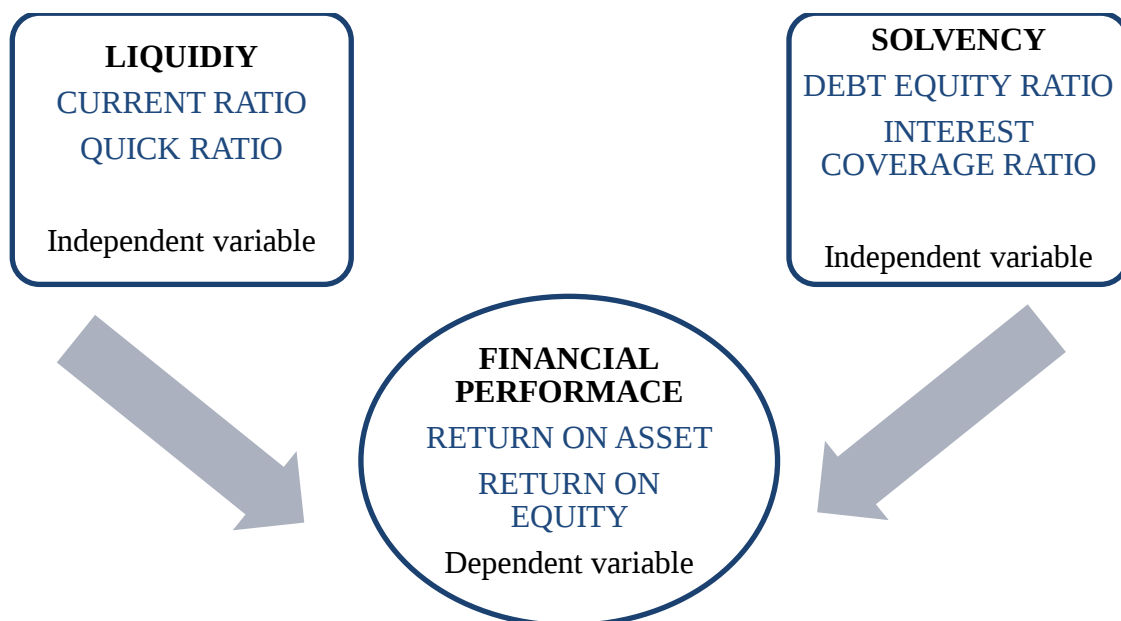
Figure 1: Quantitative Model for Multiple Regression Analysis
