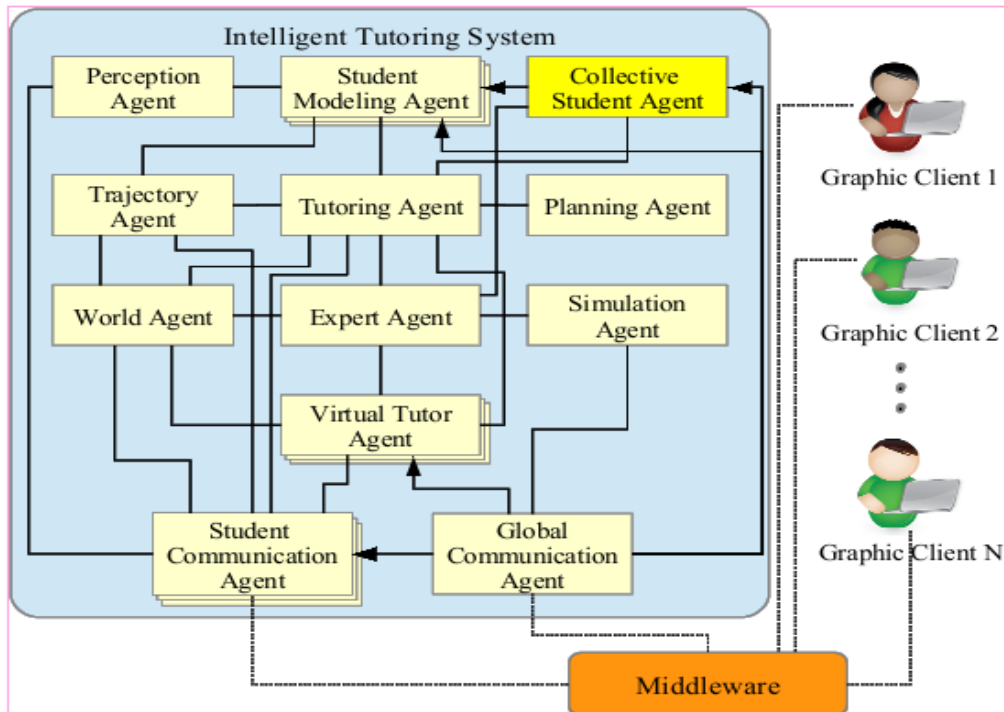
Figure 1: Administration process of Intelligent Tutoring System
